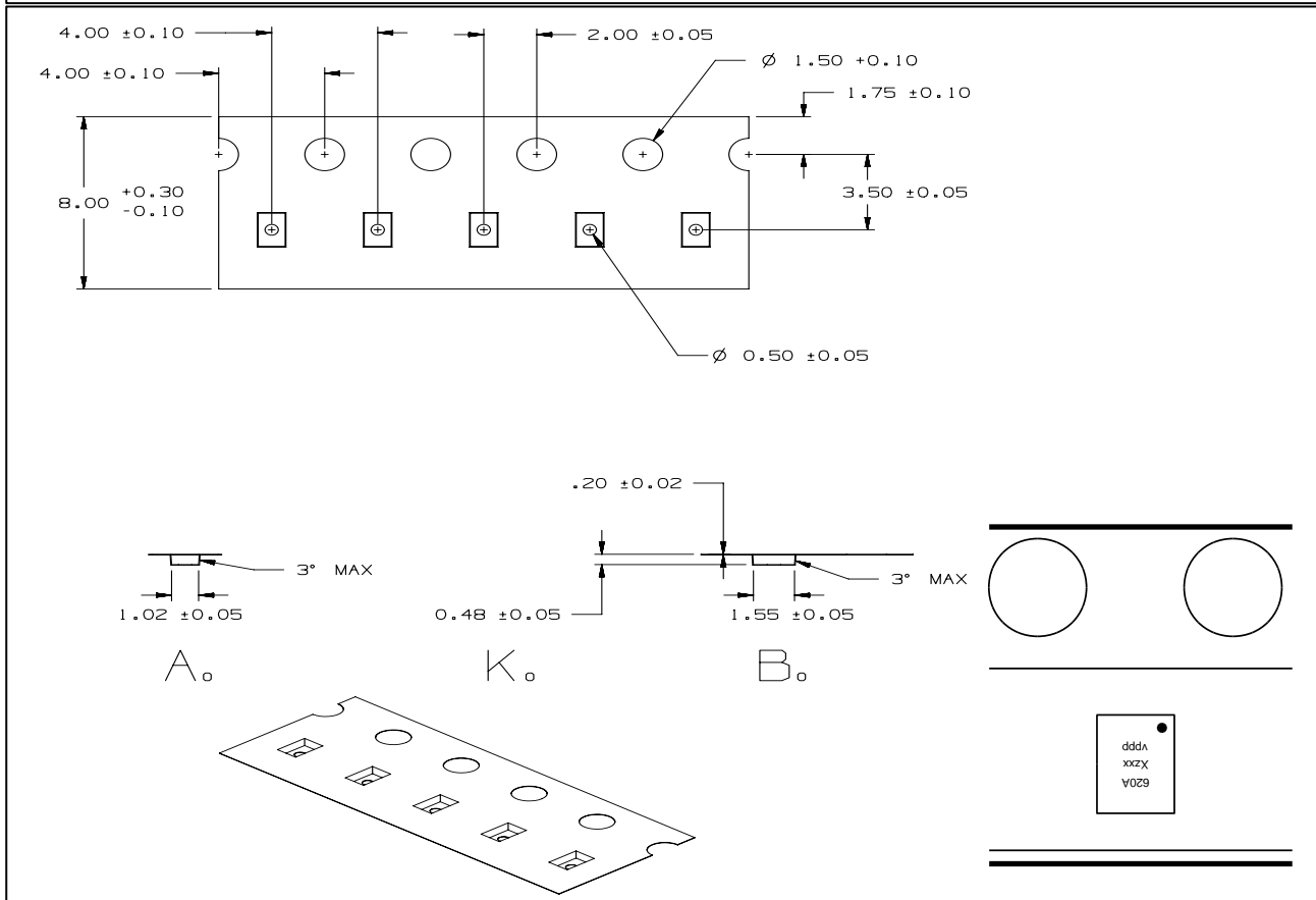
Figure 10.6 IQS620A WLCSP-9 tape & reel specification
