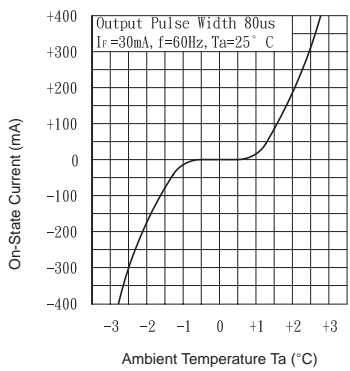
Fig.7 On-State Characteristics
