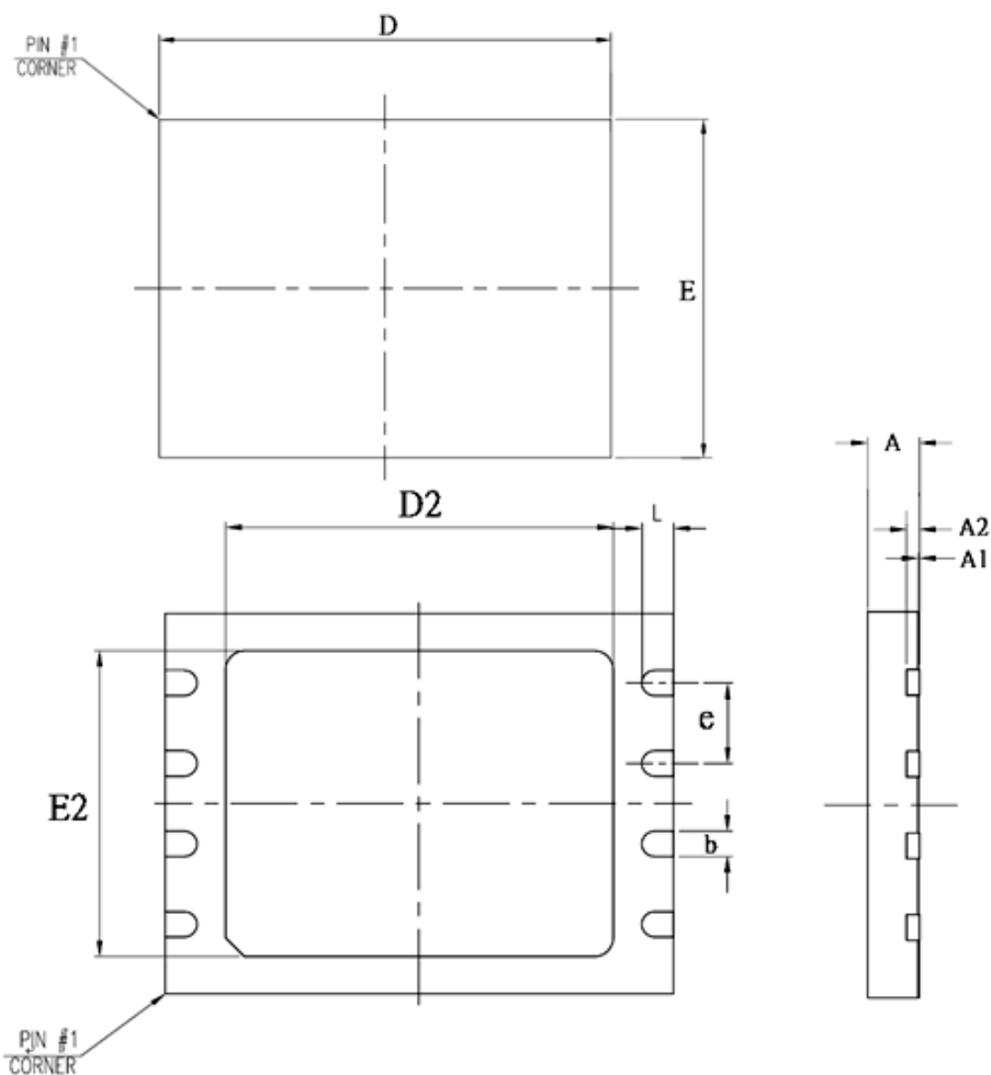
Figure 39. VDFN8 ( 5x6mm )
