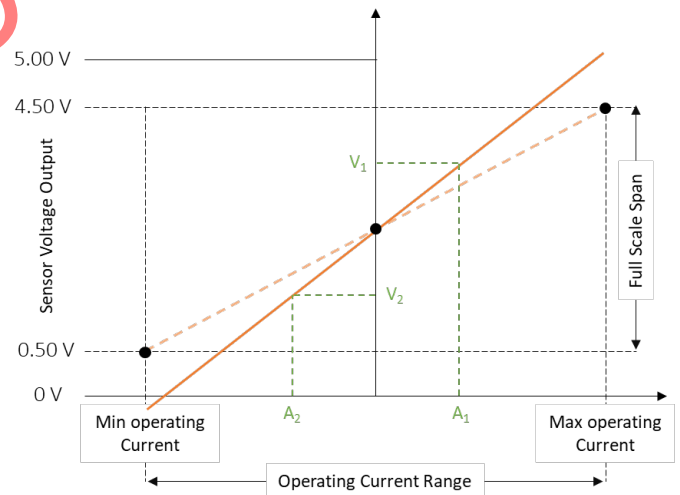
Figure 13. Gain Calibration
