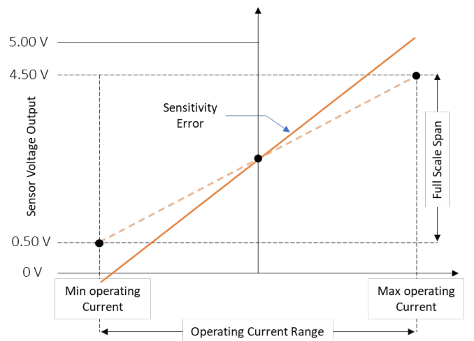
Figure 10. Exaggerated Gain Error
