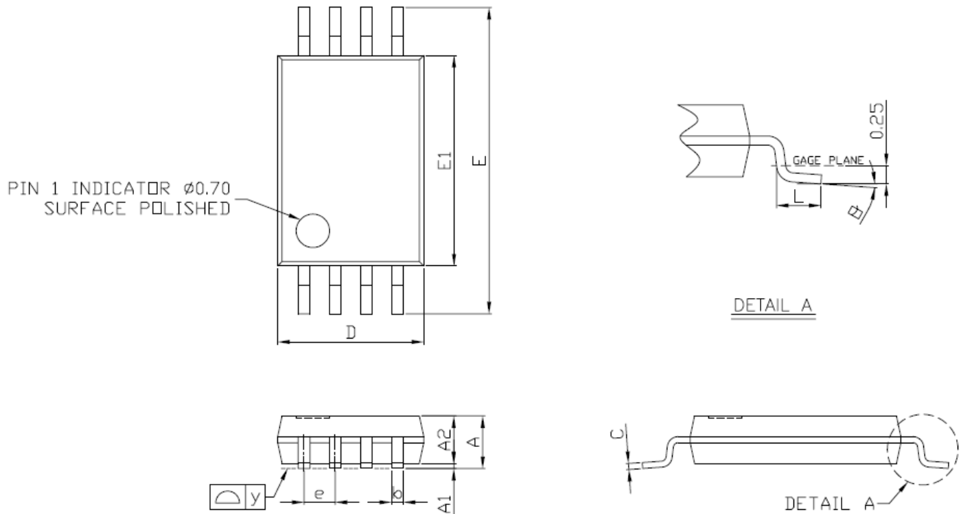
Figure 15. TSSOP-8 Package Drawing
