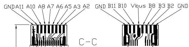
USB-C31-PLUG-C-BK-PCB-C
